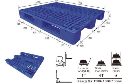
B20# C-type Pallet (can place 3pcs steel pipe)
