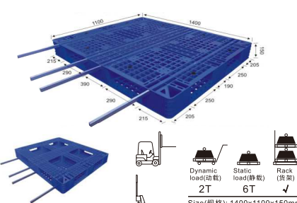
55# T-type Pallet (can place 4pcs steel pipe)
