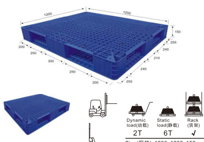
37# Double Side Pallet
