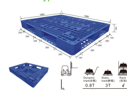
N8# T-type Pallet
