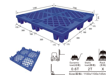
5#(flat) 9 Feet Pallet
