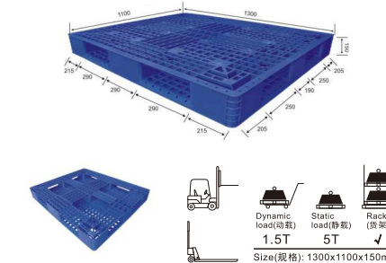
B18# T-type Pallet
