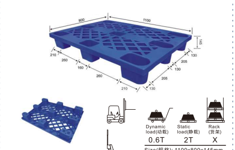
A25# 9 Feet Pallet
