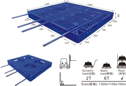
A18# T-type Pallet (can place 4pcs steel pipe)
