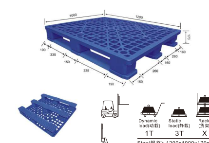
B24# C-type Pallet
