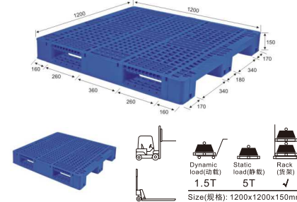
45# C-type Pallet (can place 8pcs steel pipe)
