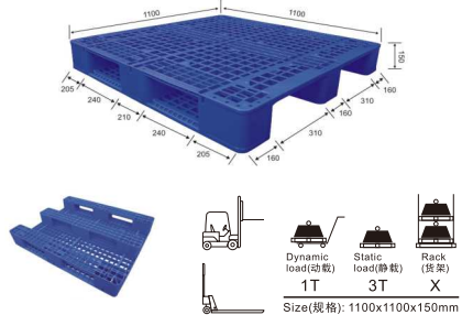
26# C-type Pallet (can place 3pcs steel pipe)
