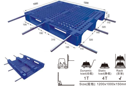
NB20# C-type Pallet (can place 6pcs steel pipe)
