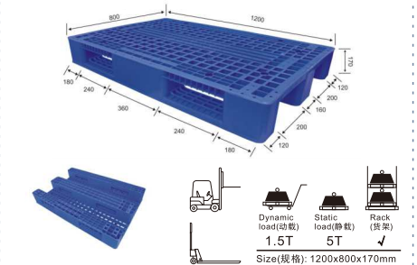
A17# C-type Pallet
