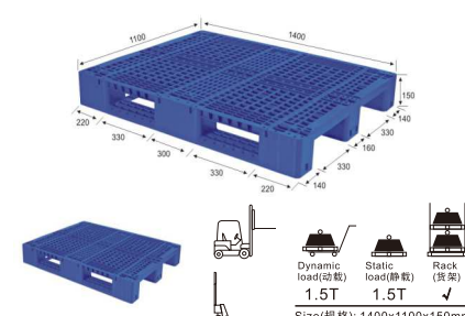
54# C-type Pallet (can place 8pcs steel pipe)
