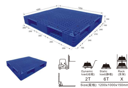
38# Double Side Pallet
