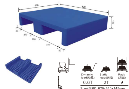
11# C-type Platform Pallet
