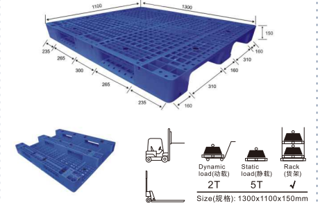
19# C-type Pallet (can place 8pcs steel pipe)
