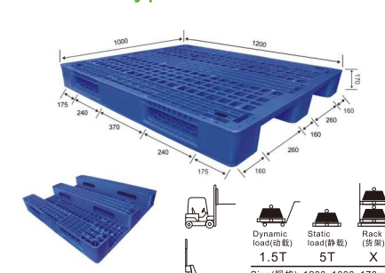
A7# C-type Pallet
