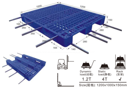
NA20# C-type Pallet (can place 8pcs steel pipe)
