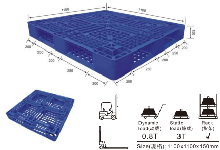
B9# T-type Pallet
