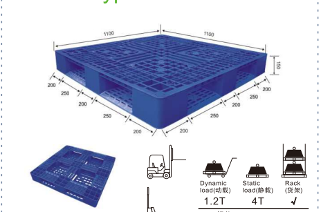
A9# T-type Pallet
