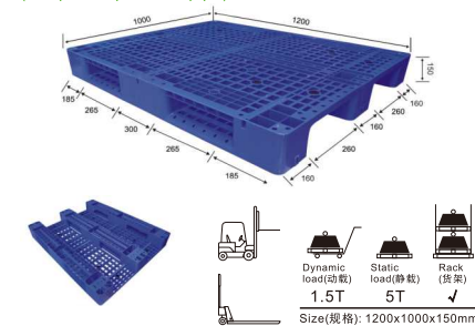
A20# C-type Pallet (can place 6pcs steel pipe)
